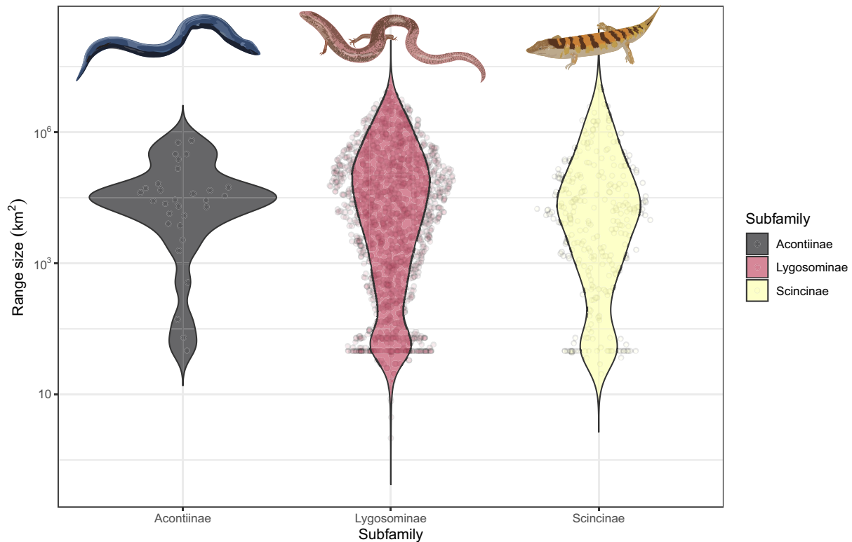
FIGURE 3 Violin plots comparing range sizes ( \log_{10} km 2 ) among the three skink subfamilies. Data from GARD 1.7 ( http://www.gardinitiaive.org/ ; Caetano et al., 2022).
